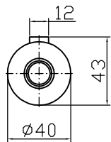
Output shaft
