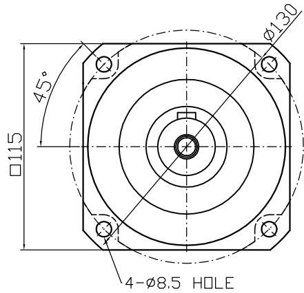
Output shaft
