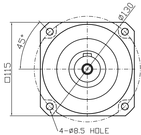
Output shaft
