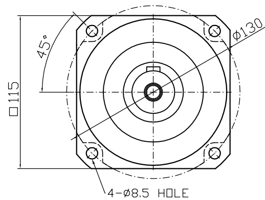
Output shaft
