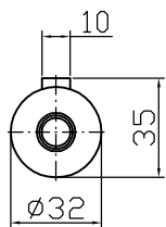
Output shaft
