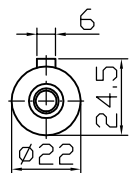
Output shaft
