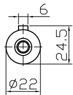
Output shaft
