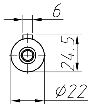
Output shaft
