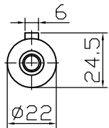
Output shaft
