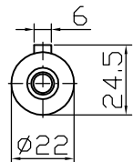
Output shaft
