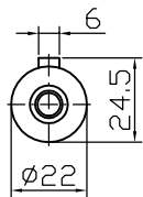
Output shaft
