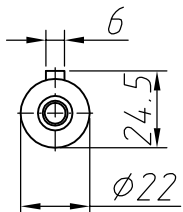
Output shaft
