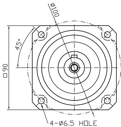
Output shaft
