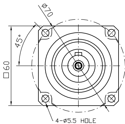
Output shaft
