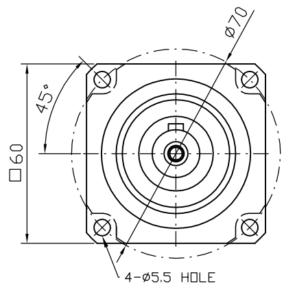
Output shaft
