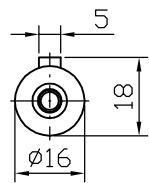
Output shaft
