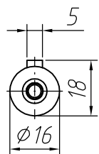
Output shaft
