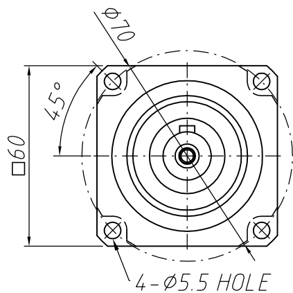
Output shaft
