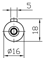
Output shaft
