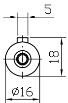
Output shaft
