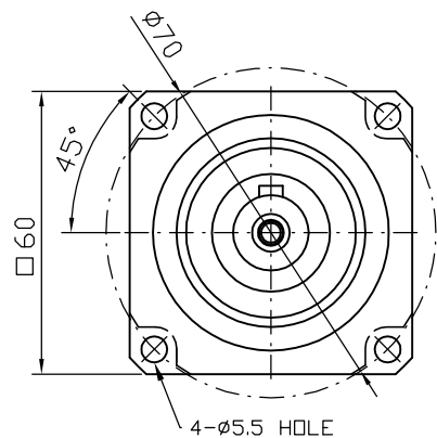
Output shaft
