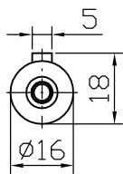
Output shaft
