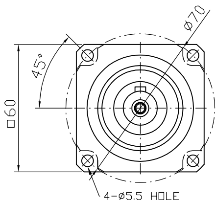
Output shaft
