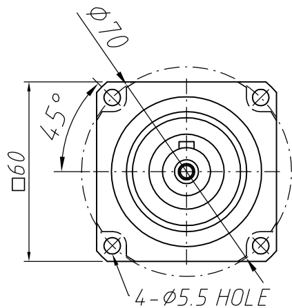
Output shaft
