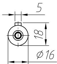
Output shaft
