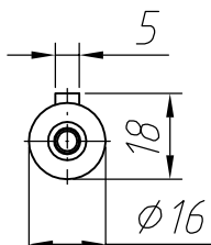
Output shaft
