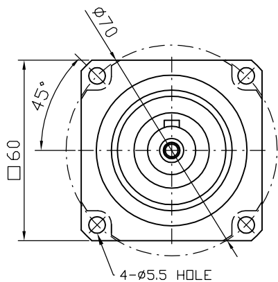
Output shaft
