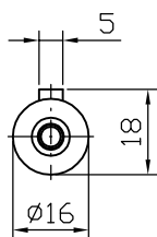
Output shaft
