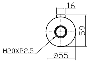
Output shaft
