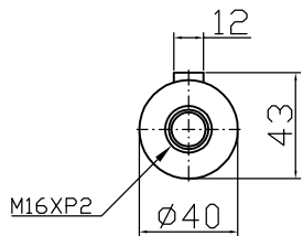
Output shaft
