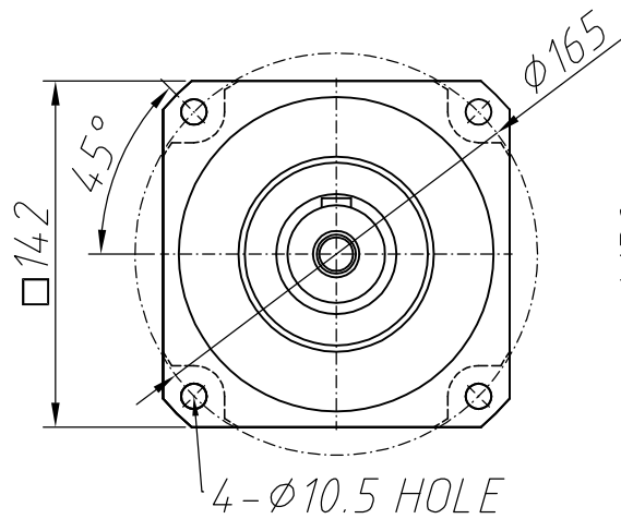
Output shaft
