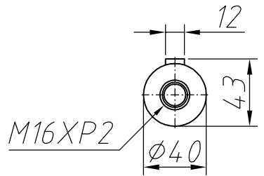
Output shaft
