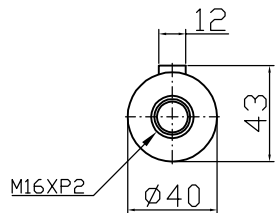
Output shaft
