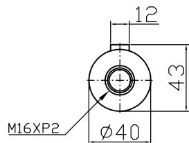
Output shaft
