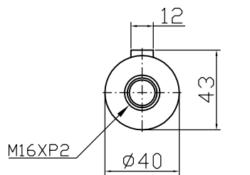
Output shaft
