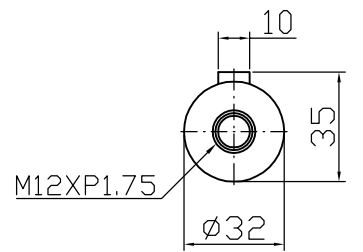
Output shaft
