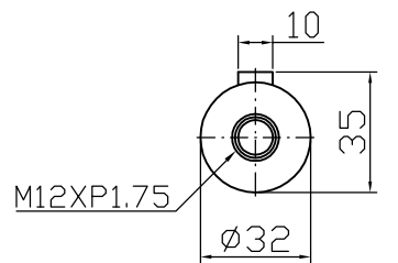
Output shaft
