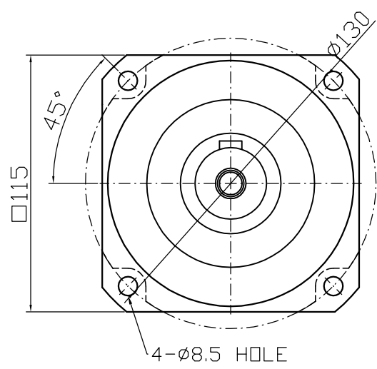
Output shaft
