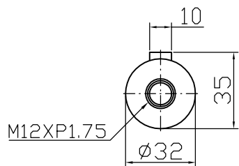
Output shaft
