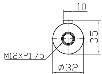
Output shaft
