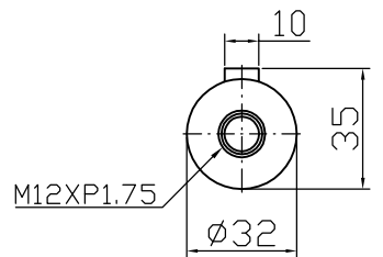
Output shaft
