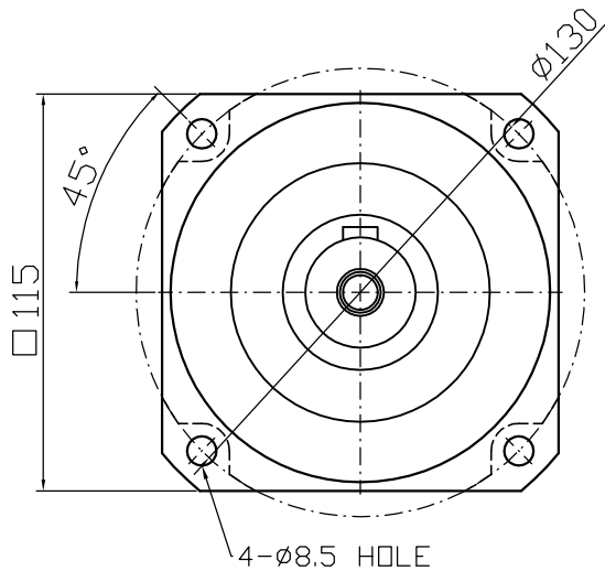
Output shaft
