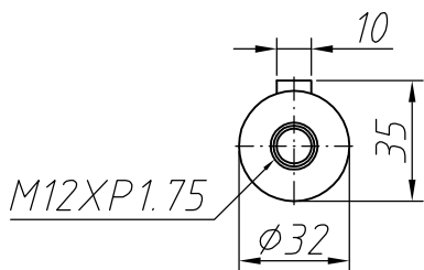
Output shaft
