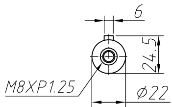
Output shaft
