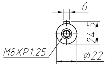
Output shaft
