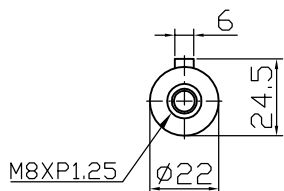
Output shaft
