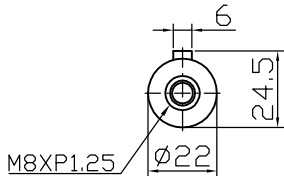
Output shaft
