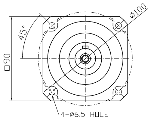
Output shaft
