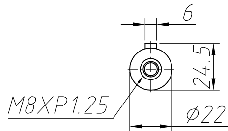
Output shaft
