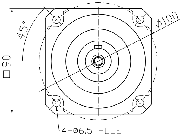
Output shaft
