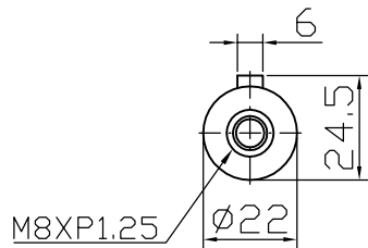
Output shaft
