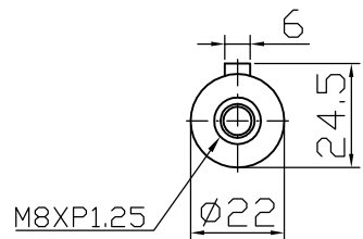
Output shaft
