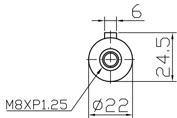
Output shaft
