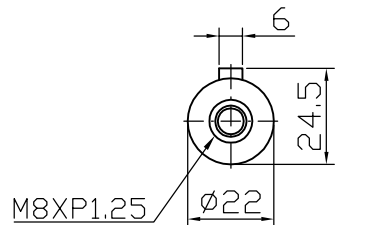
Output shaft
