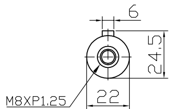
Output shaft
