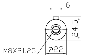
Output shaft
