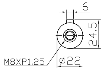
Output shaft
