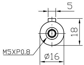
Output shaft
