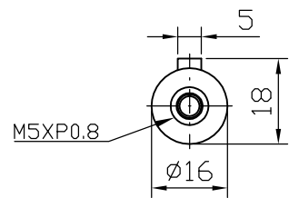
Output shaft
