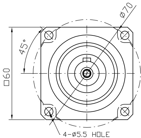
Output shaft
