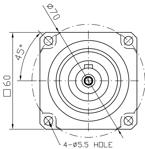
Output shaft
