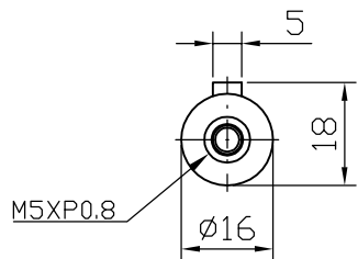
Output shaft
