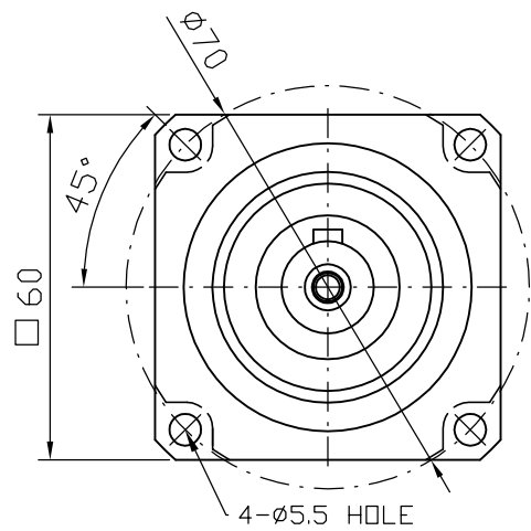
Output shaft
