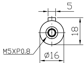
Output shaft
