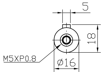
Output shaft
