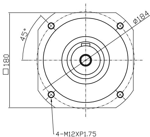
Output shaft
