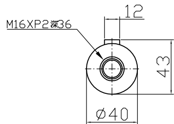
Output shaft
