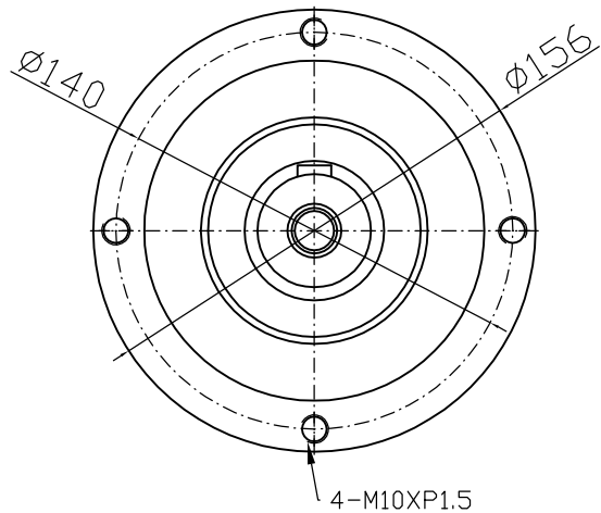
Output shaft
